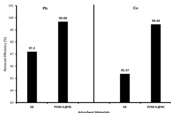
Figure 4: Heavy metals removal properties of NC and POM-IL@NC materials. Pollutant concentration: Pb = 2.2 mM, Cu = 1.4 M; WHO limit: Pb = 0.01 mg/L (0.048 µM), Cu = 2 mg/L (32 µM) 22
